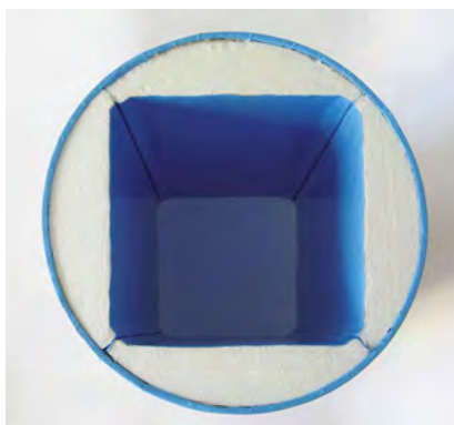
PANATUB Casseri in cartone rettangolari / quadrati PANATUB Baurohre rechteckig / quadratisch PANATUB Rectangular / square tubular formwork
